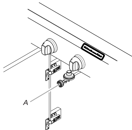
A. Gas pressure regulator/hose assembly
