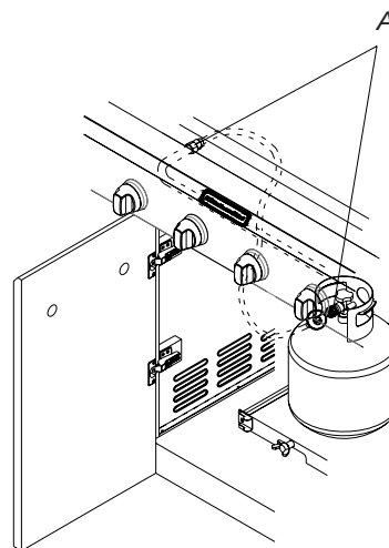
A. Gas pressure regulator/hose assembly
