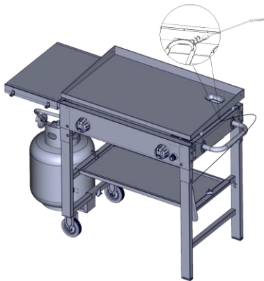
Main Burner
