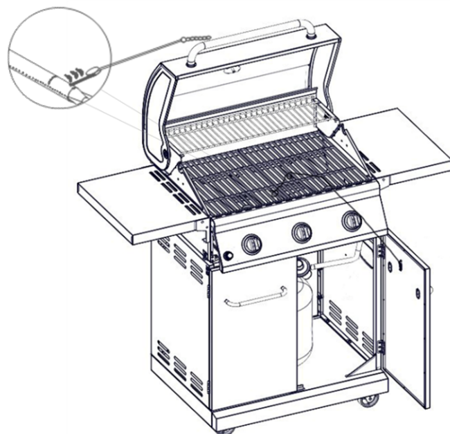
Main burner
