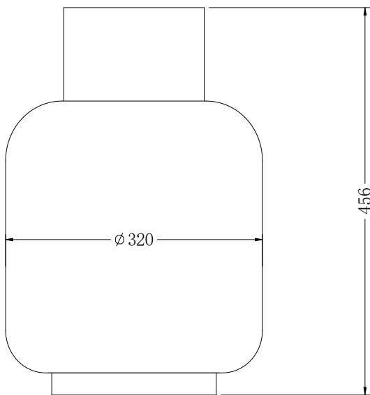
Propane tank: height = 456mm, diameter = 320mm
