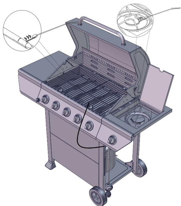
Main Burner
